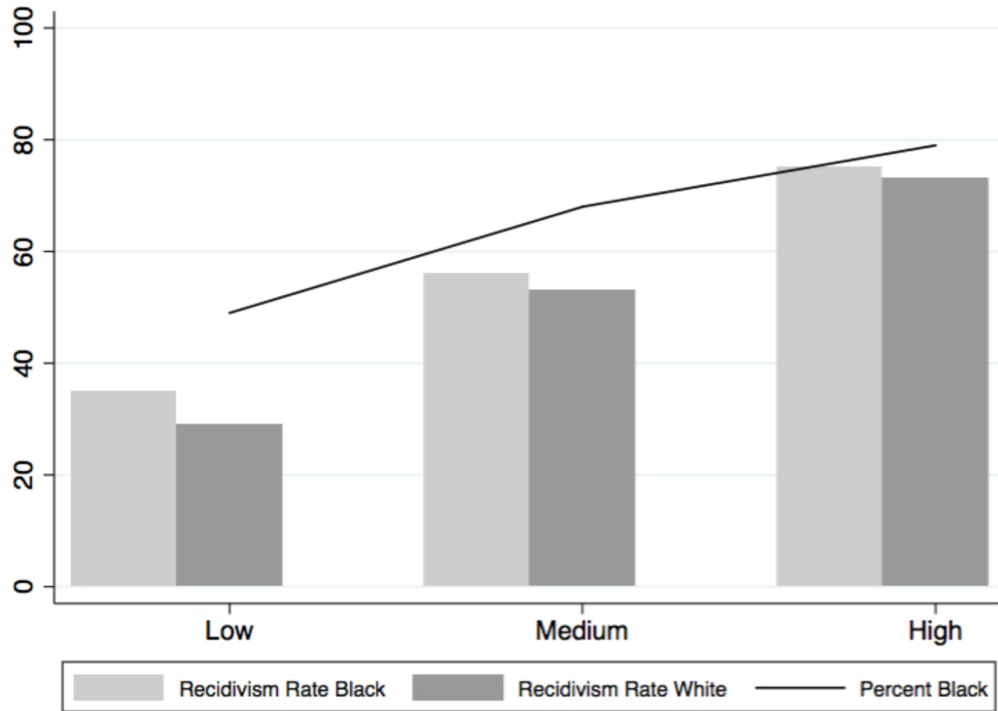
Figure 3. Recidivism Rates by Race and Percent Black in Each Risk Category—Any Arrest
