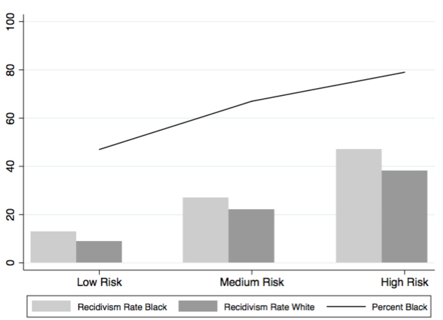
Figure 4. Recidivism Rates by Race and Percent Black in Each Risk Category—Arrest Violent Offense
