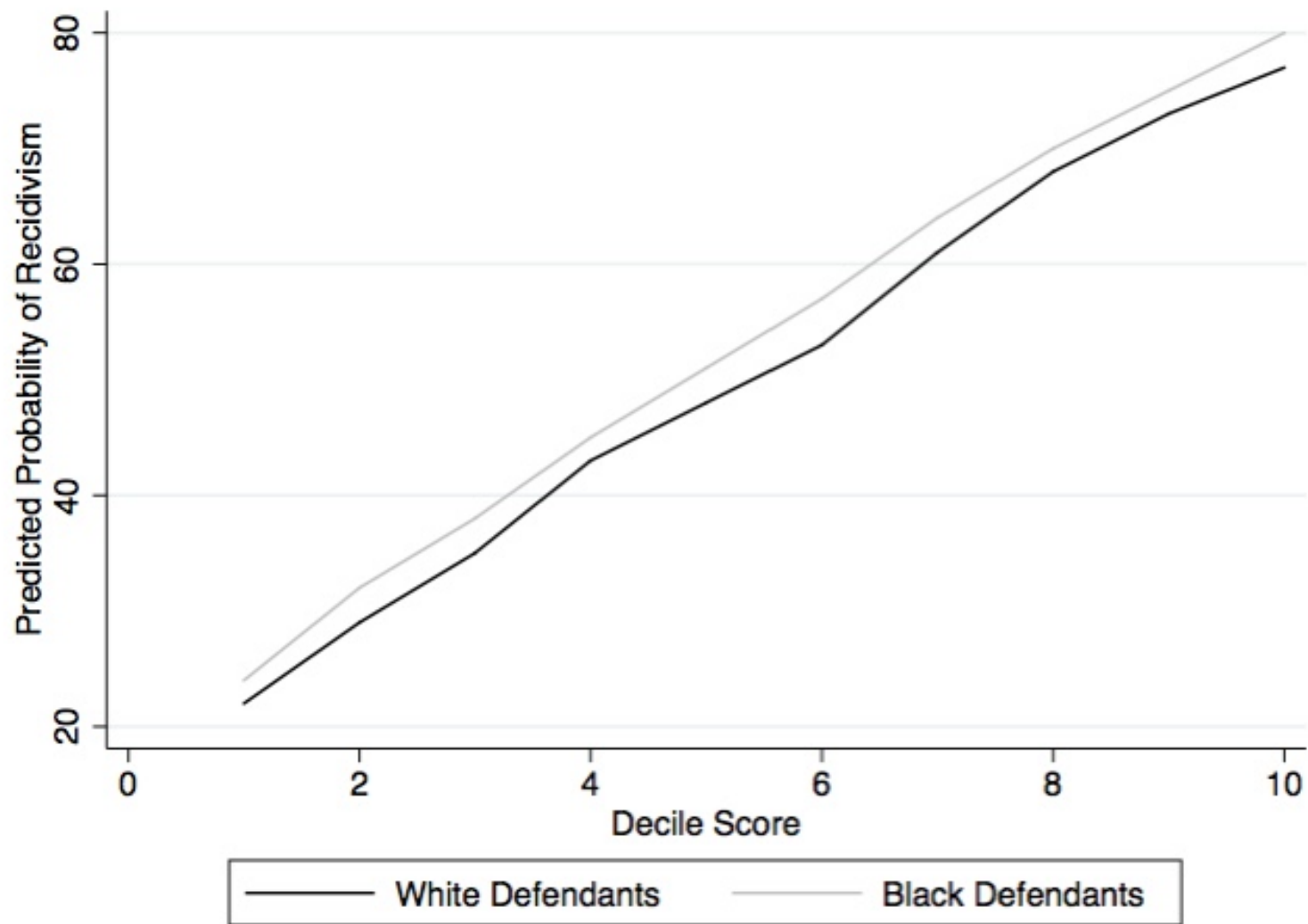
Figure 1. Predicted Probability of Any Arrest by Race
